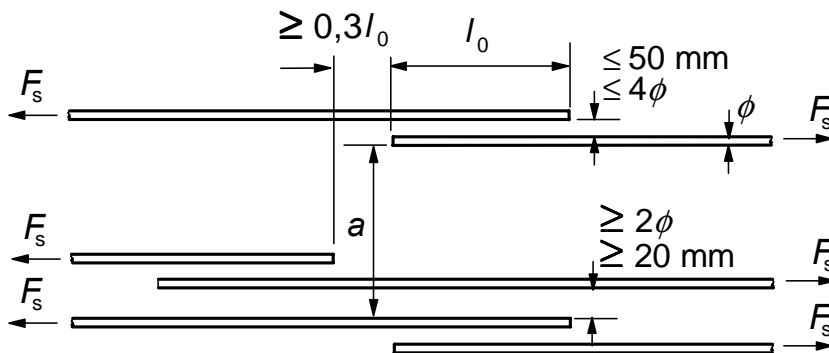
Figure 8.7: Adjacent laps
