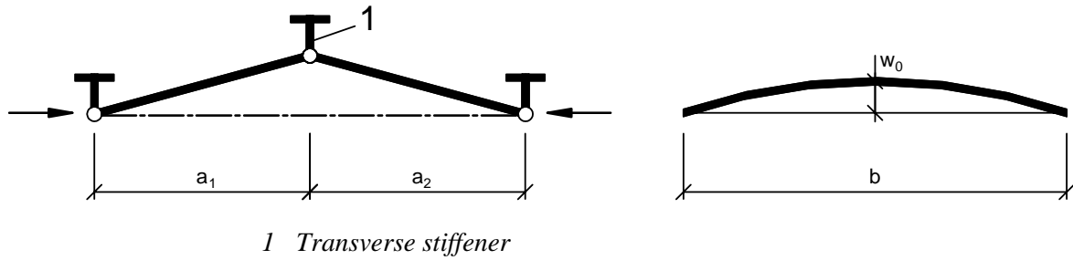
Figure 9.2: Transverse stiffener
