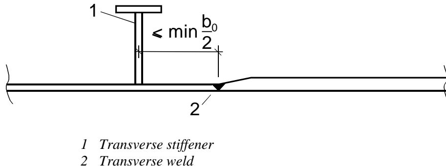
Figure 9.3: Welded plates
