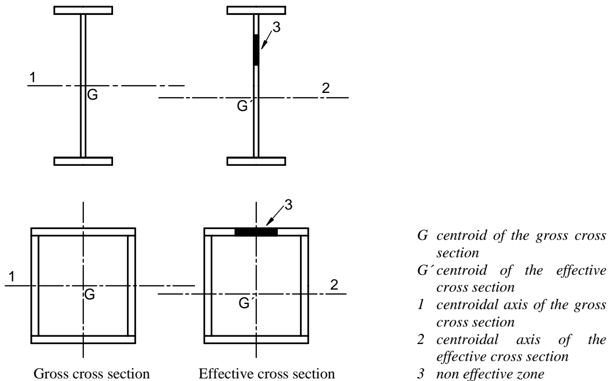
Figure 4.2: Class 4 cross-sections - bending moment
