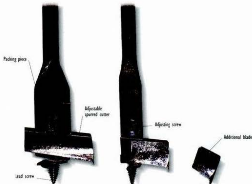
ABOVE: A large size expanding bit
