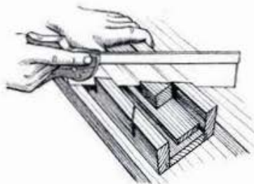
ABOVE: Miter jig. The strip of waste wood under the workpiece saves the jig from saw damage.
