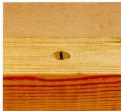
ABOVE: If all is well, the top face of the screw will be a clean fit, but fractionally lower than the surface of the wood.
