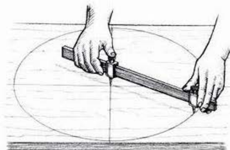
ABOVE: Spike one trammel point down on the center and swing the other point to scribe the circle.
