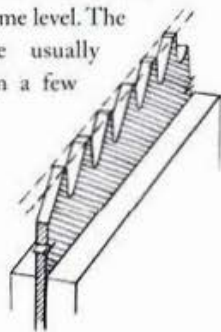
RIGHT: Jointing the rip saw.
