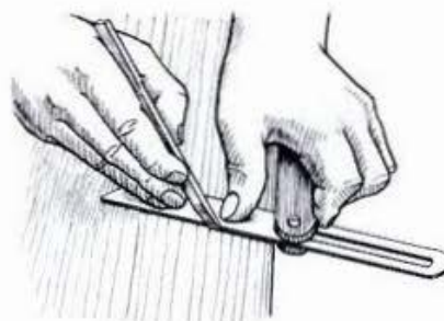
ABOVE: It is important to make sure that the wooden stock of the bevel is held hard up against the edge of the workpiece.
