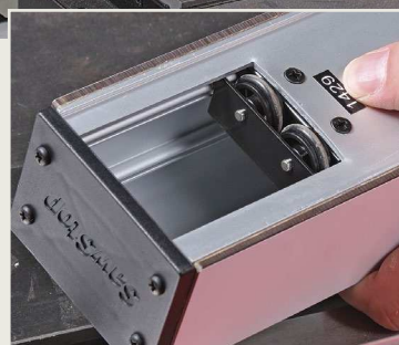
Slick fence. Sturdy and deflection-free, the SawStop’s fence locks down tight (above). It also glides over the table as if it were floating on air, thanks to a pair of small wheels at the end (left).
