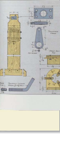
Clamp up from yellow pine framing lumber. Each wooden lathe cost less than $200 in materials. With its 1½-ft. bed, it can handle up to 8-ft. work. A strip of wood, secured by the head through drilled holes, activates the on/off switch from anywhere on the bed.
