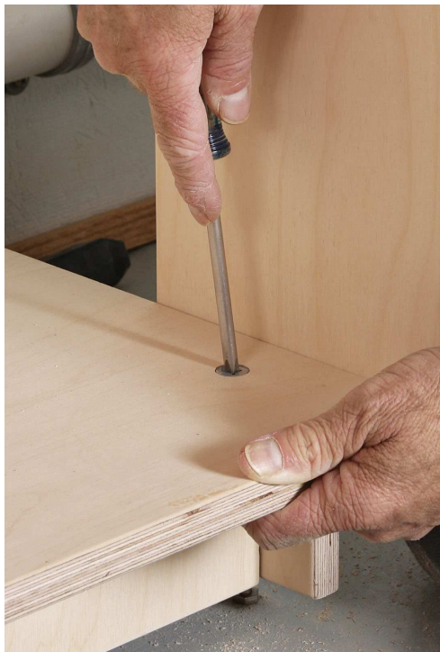
Lock it in. As you turn the cam in the shelf, the pin and leg are pulled tight, creating a rigid base for the top.
