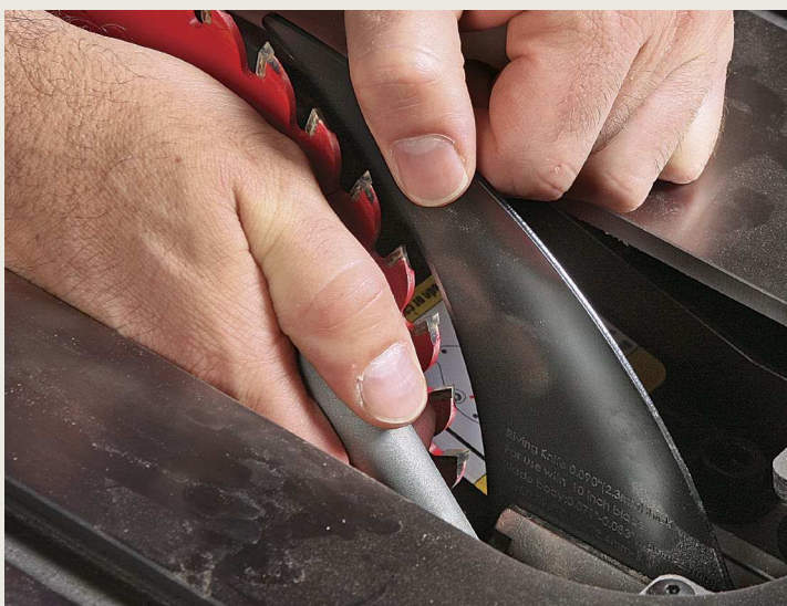
Quick exchange from riving knife to guard. A big, easy-to-reach lever is all you need to free them on the SawStop.
