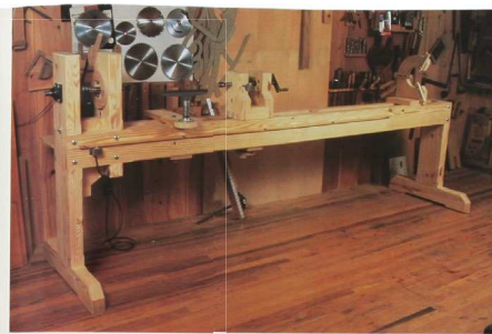
Clamp up from yellow pine framing lumber. Each wooden lathe cost less than $200 in materials. With its 1½-ft. bed, it can handle up to 8-ft. work. A strip of wood, secured by the head through drilled holes, activates the on/off switch from anywhere on the bed.
