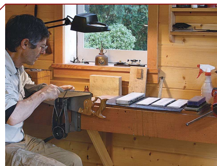
Get sharp. Along with his ceramic stones and diamond plate, which live on a rubber mat, Tolpin’s wall-mounted sharpening bench features a saw-sharpening vise and a task lamp with a magnifying lens.
