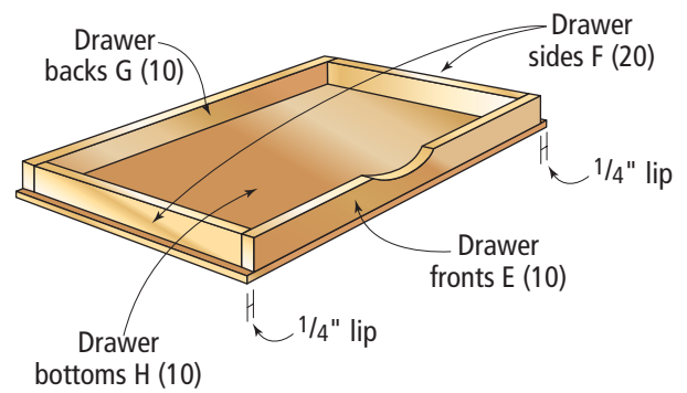
Drawer assembly
