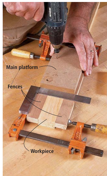
To assemble a lapping platform, capture a workpiece between the fences and align the primary platform on them. The edge of the platform must be square to the work. You can build the simple version of this jig for cross-laps as shown in the photo or add a work stop as shown in the illustration to also cut end-laps.
