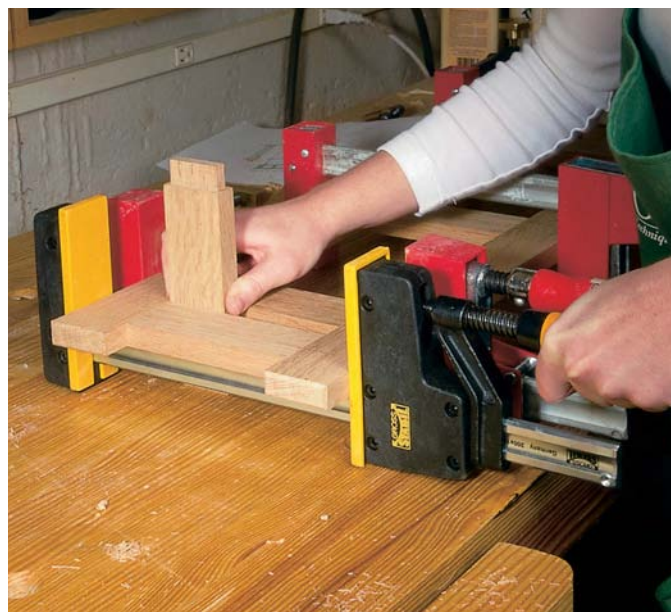
Slide an extra rail (which is \frac{3}{4} " thick) into the space between the top two rails to ensure a perfect slot for the top shelf.
