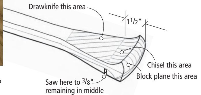
Chisel a hollow approaching the saw kerf. Beware that two cut lines like this can be difficult to blend smoothly. Before cutting too far, expect to clean it up with a rasp and sandpaper.
