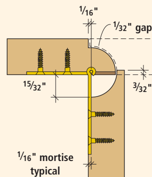
Hinge detail
