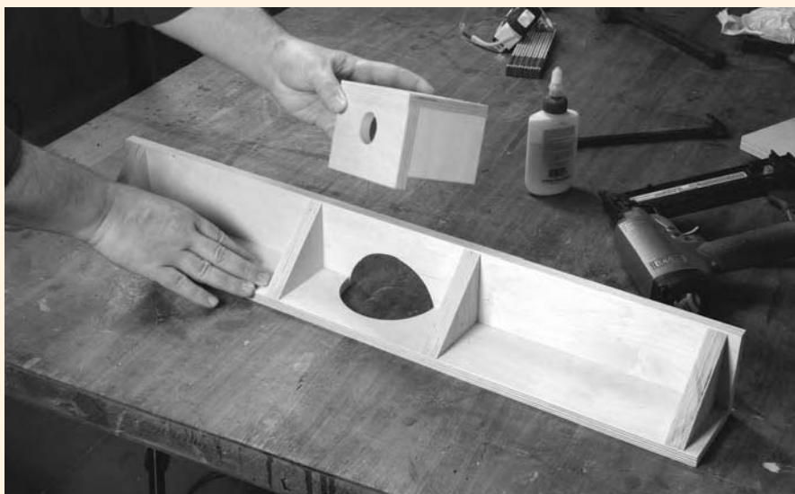
Dust collection can be designed right into jigs and fixtures. This router fence includes a tightly fitted dust-collection hood for efficient pickup.
