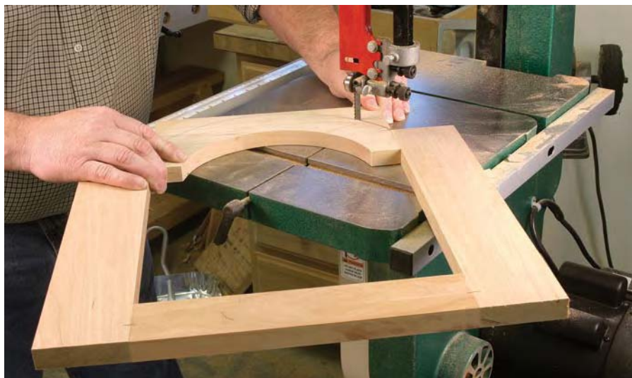
Fit the hood door. Once the outer arch is cut, the door is fit to the hood. Fit the door in position then fine-tune the fit to create an even reveal around the door.
