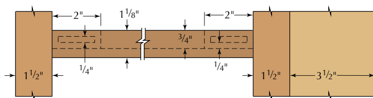
FACE-FRAME-TO-DRAWER-RUNNERS JOINERY
