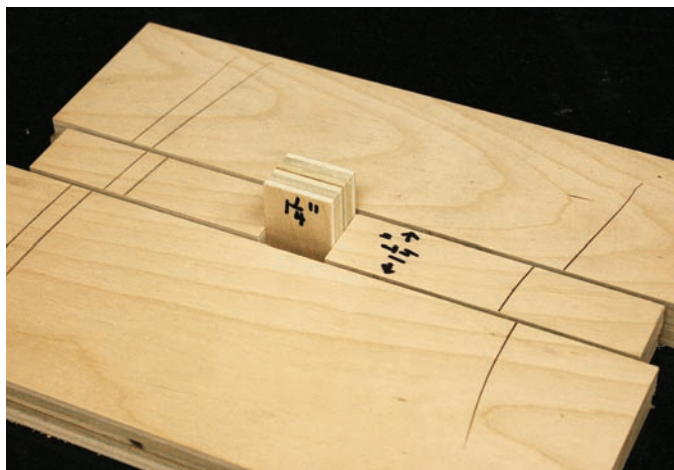
Cheap insurance. The small block turned sideways fixes the same distance between the center strips as the width of the strips. Be sure not to glue the spacer block in place—but leave it there until the glue dries.
