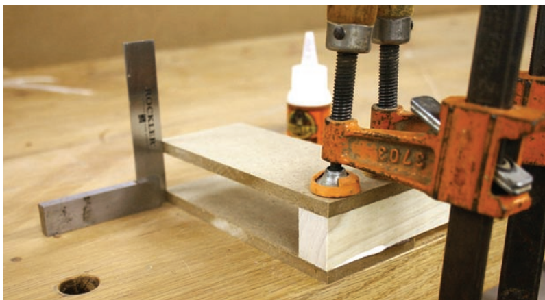
Both sides the same. When gluing the marking jig it is critical that the sides are square and parallel to one another. After the glue dries I always check them and true them up on my edge sander, if needed.
