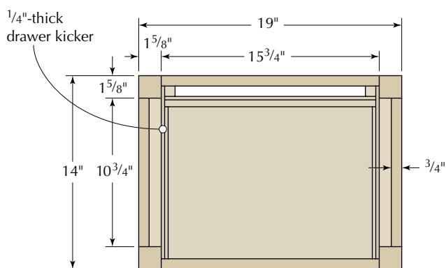
SECTION THROUGH DRAWER
